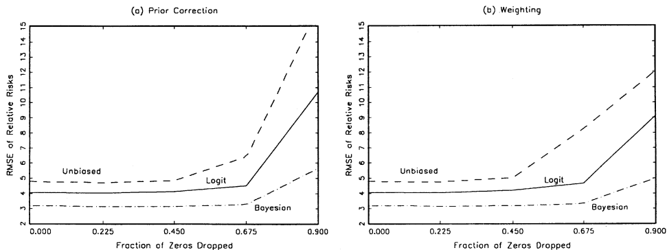
Fig. 9 RMSE of relative risk estimates: subsampled data.
