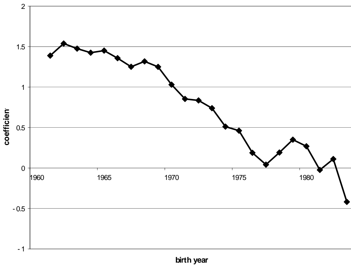
Coefficients for Time Dummies in the Final Model
