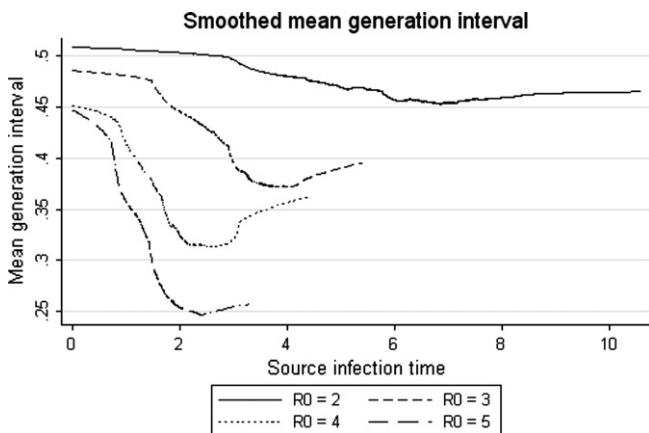
Fig. 2. The smoothed mean generation interval as a function the source infection time for R_0 = 2, 3, 4, 5 . There is a clear tendency to contract, with greater contraction for higher R_0 .
