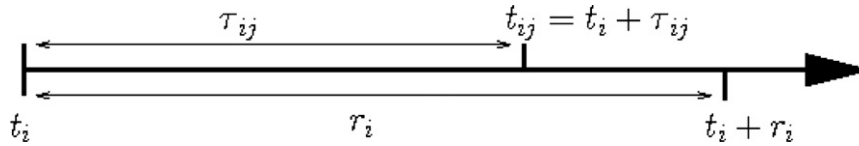
Fig. 1. Schematic diagram of variables in the general stochastic SIR model for the ordered pair ij . Recall that t_j \leq t_{ij} . As discussed in Section 3.2, person i develops symptoms at time t_i^{sym} = t_i + q_i , where q_i is the incubation period.
