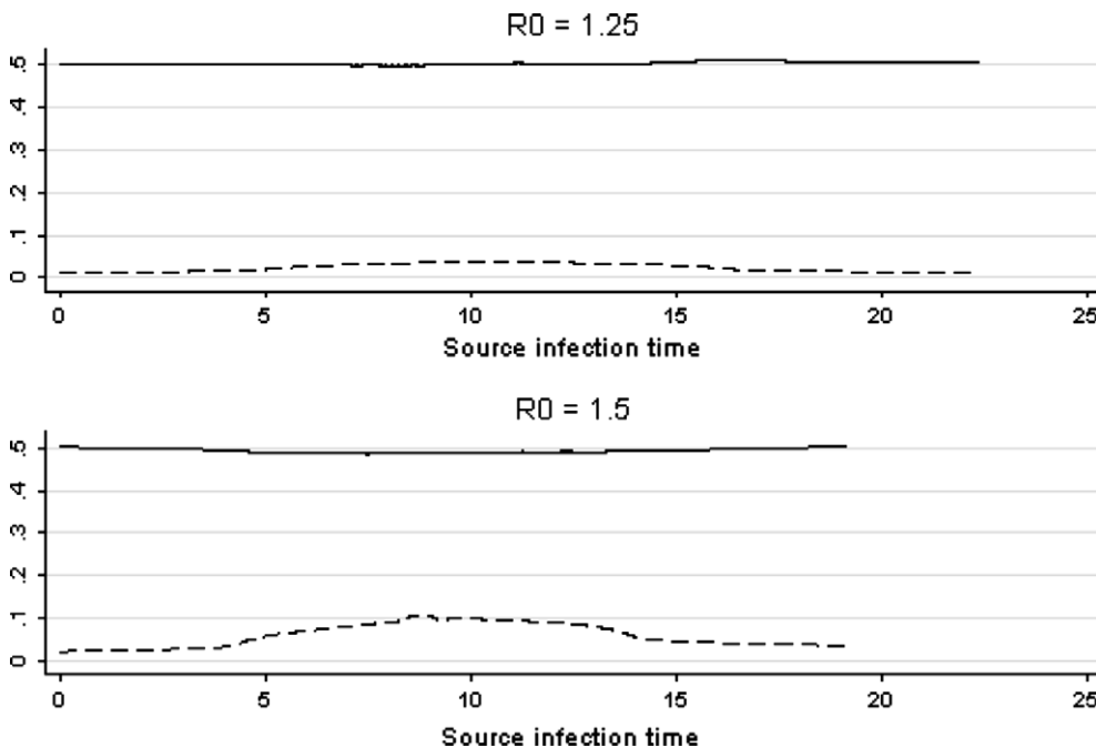
Fig. 4. The smoothed mean generation intervals (solid lines) and prevalence (dotted lines) as a function of the source infection time for R_0 = 1.25 and 1.50 . For R_0 near one, the mean generation interval stays relatively constant.
