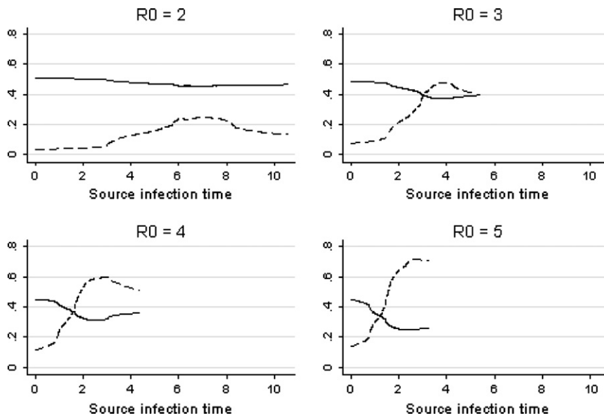
Fig. 3. The smoothed mean generation interval (solid lines) and prevalence (dotted lines) as a function of the source infection time for R_0 = 2, 3, 4, 5 . In all cases, the greatest contraction of the serial interval coincides with the peak prevalence of infection (i.e., the greatest competition among potential infectors).
