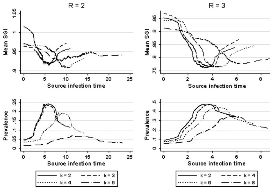
Fig. 5. The smoothed mean scaled generation interval (SGI) and prevalence as a function of the source infection time for R = 2 and R = 3 . With increasing cluster size, the degree of generation interval contraction is roughly the same even though the peak prevalence of infection is lower.
